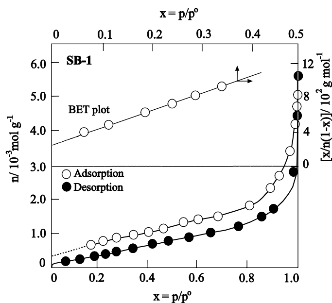
Figure 6. The adsorption-desorption isotherms and BET plot of OBs SB-1.
