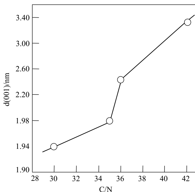
Figure 5. The change in the basal spacing of the C/N molar ratio.
