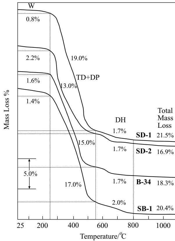
Figure 4. TGA curves of the OBs (W: interparticle water; TD: thermal degradation; DP: degradation products; DH: dehydroxylation; DS: decrystallization of smectite).
