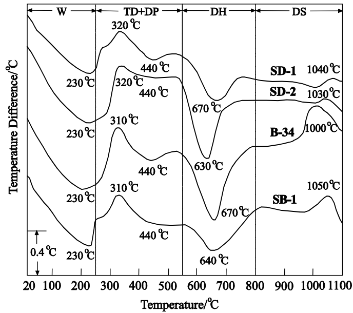
Figure 3. DTA curves of the OBs (W: interparticle water; TD: thermal degradation; DP: degradation products; DH: dehydroxylation; DS: decrystallization of smectite).
