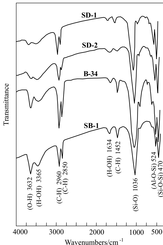
Figure 2. FTIR spectra of the OBs.
