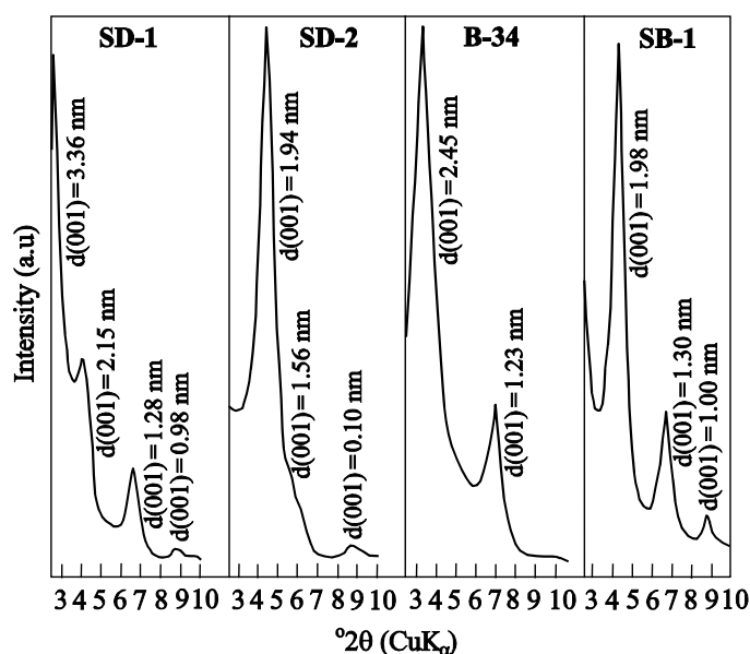
Figure 1. XRD patterns of the OBs.
