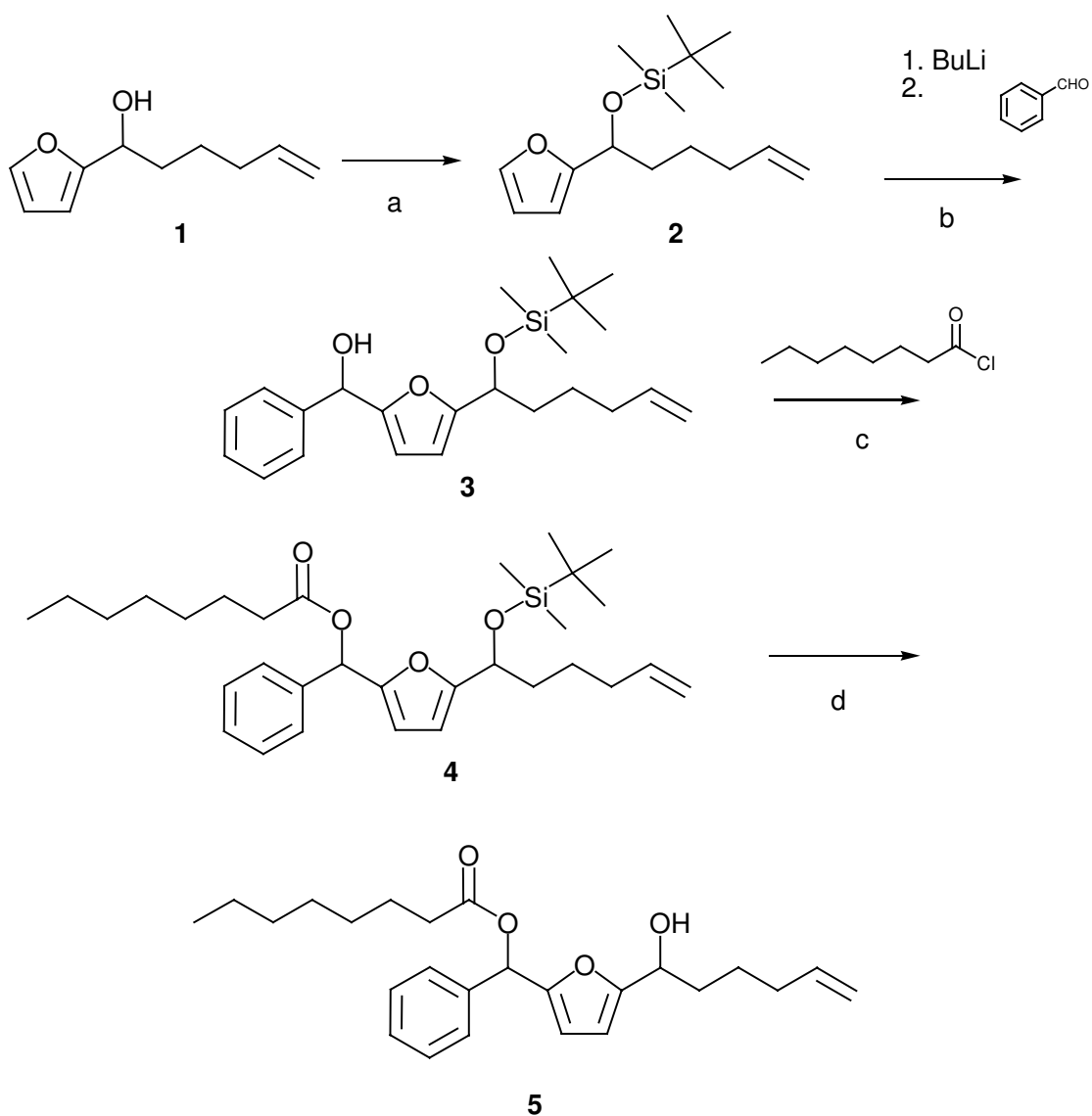
Scheme 1. THF, TBDSCl, imidazole b. THF, -40^\circ\text{C} , c. toluene, \text{NEt}_3 , d. THF, \text{NBu}_4\text{F} .
