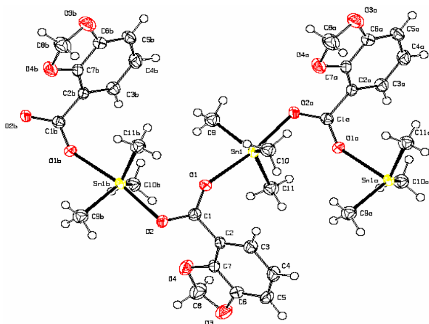
Figure 2. An ORTEP [18] drawing of complex 1 . Displacement ellipsoids are drawn at 50% probability level.
