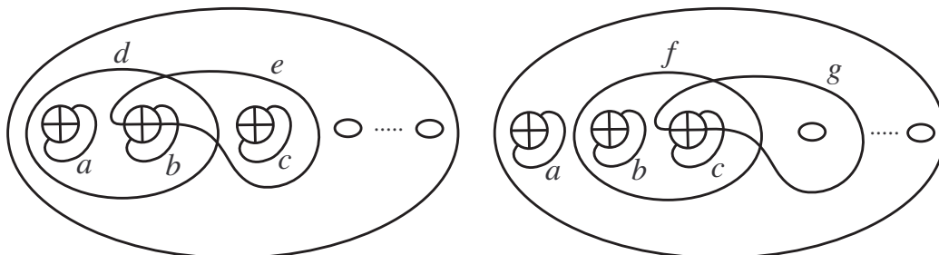
Figure 9. Some curves on genus 3 surface with boundary.
