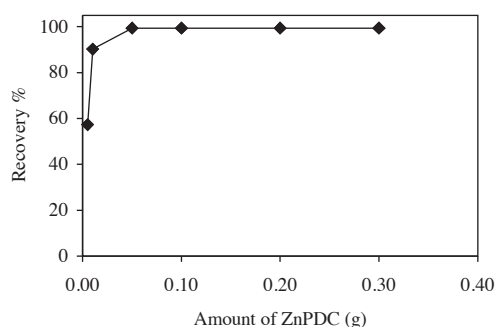
Figure 3. Effect of the amounts of ZnPDC on the recovery of cadmium. Oil standard: 1.00 g, n-hexane: 3 mL, back-extraction: 10 mL of 0.1 mmol mL -1 Hg(II). (N: 3).
