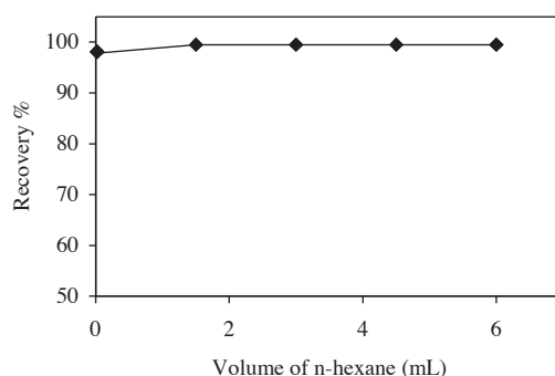
Figure 4. Effect of volume of n-hexane on the recovery of cadmium. Oil standard: 1.00 g, ZnPDC: 0.10 g. Back-extraction: 10 mL of 0.1 mmol mL -1 Hg(II). (N: 3).
