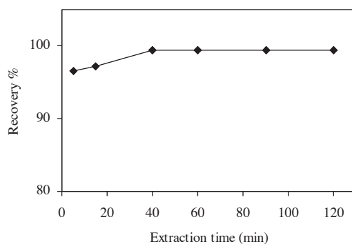
Figure 5. Effect of extraction time on the recovery of cadmium. Oil standard: 1.00 g, n-hexane: 3 mL, ZnPDC: 0.10 g. Back-extraction: 10 mL of 0.1 mmol mL -1 Hg(II). (N: 3).
