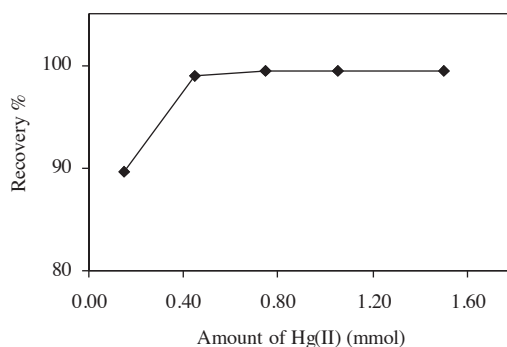
Figure 7. Effect of amount of Hg(II) on the recovery of cadmium. Oil standard: 1.00 g, n-hexane: 3 mL, ZnPDC: 0.10 g. Extraction time: 45 min. Back-extraction time: 45 min. Volume of Hg(II): 10 mL containing different amounts of Hg(II). (N: 3).
