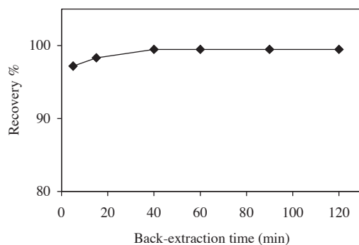
Figure 6. Effect of back-extraction time on the recovery of cadmium. Oil standard: 1.00 g, n-hexane: 3 mL, ZnPDC: 0.10 g. Extraction time: 45 min. Back-extraction: 10 mL of 0.1 mmol mL -1 Hg(II). (N: 3).
