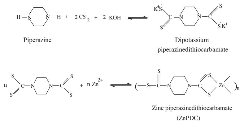
Figure 1. Preparation of ZnPDC.
