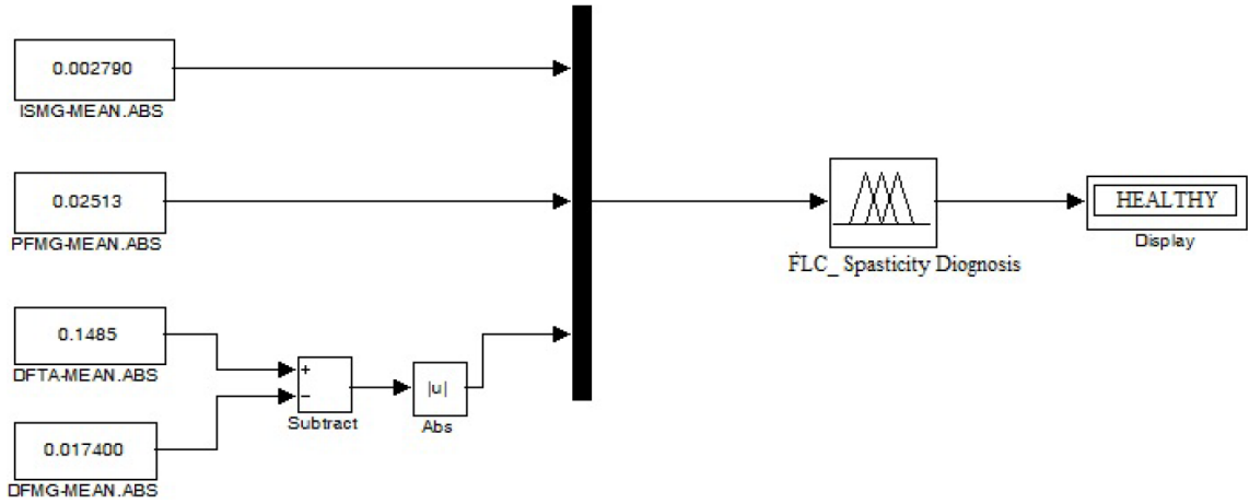
Figure 5. The FLC system.
