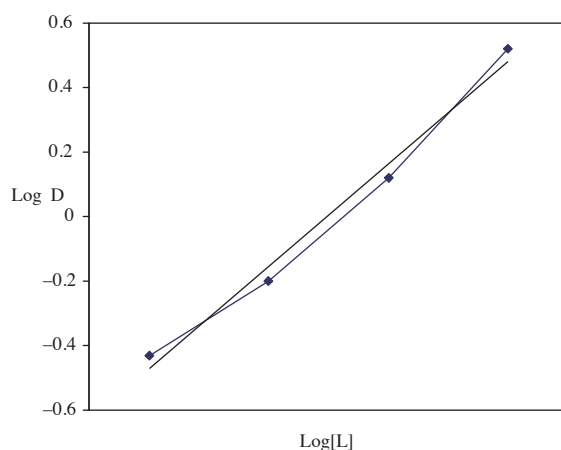
Figure 2. Log D versus log[L] for the extraction of \text{Hg}^{2+} picrates by ligand 3 from an aqueous phase into dichloromethane at 25 °C.
