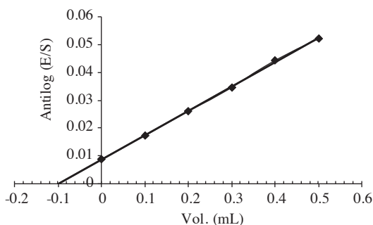
Figure 6. Plot of antilog (E/S) versus the volume of 0.1 M standard promethazine by MSA using DBPH electrode.
