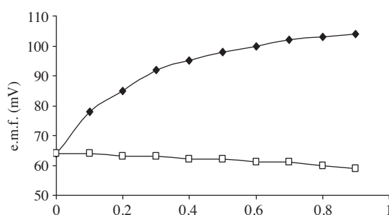
Figure 4. Selectivity of DBPH electrode for interfering \text{Cr}^{3+} by separate method, □- promethazine hydrochloride solution, ▲- solutions of \text{Cr}^{3+} .
