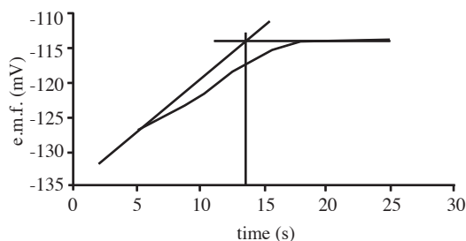
Figure 3. Plot the response time of DBPH electrode using 10^{-3} M promethazine hydrochloride.
