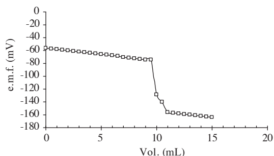
Figure 7. Titration curve of DBPH electrode for 10^{-3} M promethazine titrated with 10^{-3} M phosphotungstic acid.
