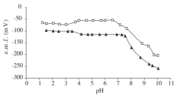
Figure 2. Effect of pH on electrode response using based on DBPH electrode. □- 10^{-2} M, ▲- 10^{-3} M promethazine-HCl.
