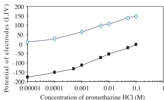
Figure 1. Calibration curves of promethazine hydrochloride selective electrodes. ◇- DBP, ■- DBPH.
