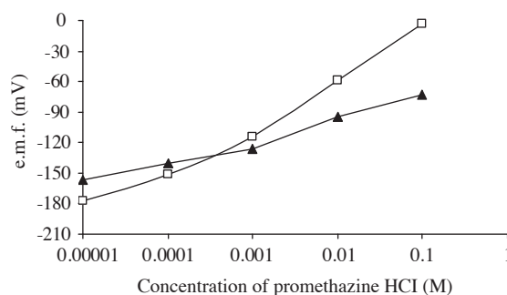
Figure 5. Selectivity of DBP electrode at 10^{-3} M promethazine-HCl in the presence of \text{Fe}^{+3} using the match method. ▲- promethazine hydrochloride solutions, □- solutions of \text{Fe}^{+3} ion.
