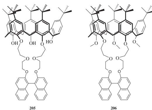
Figure 33. Chiral calix[5]arenes bearing a binaphthyl crown unit at the lower rim.
