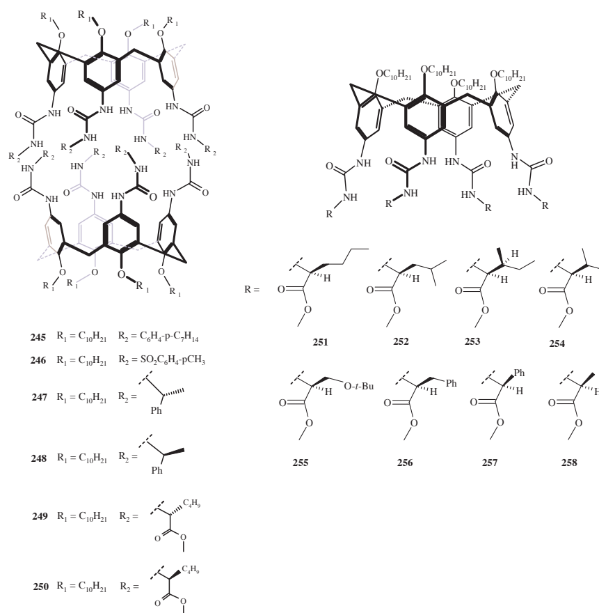
Figure 40. Tetraureas of calix[4]arene derivatives and calixarene-based dimers.
