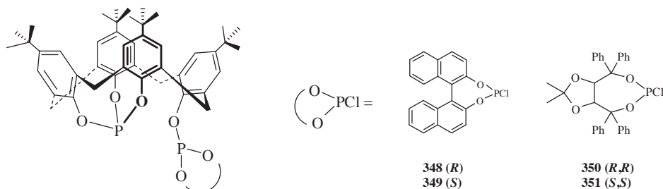
Figure 62. Chiral calixarene-based diphosphite ligands.
