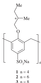
Figure 2. p -sulfonatocalix[n]arenes bearing ( S )-2-methylbutoxy groups.
