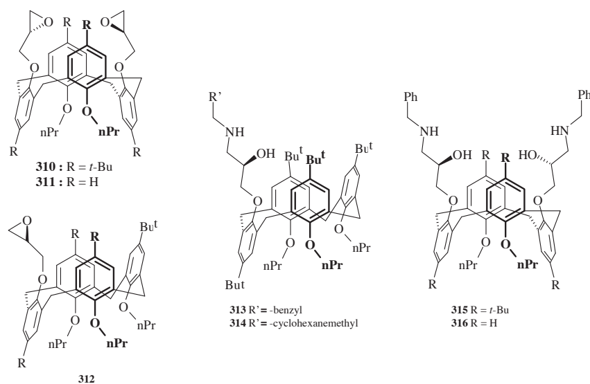
Figure 50. Chiral calix[4]arenes bearing glycidyl groups as chiral catalysts.
