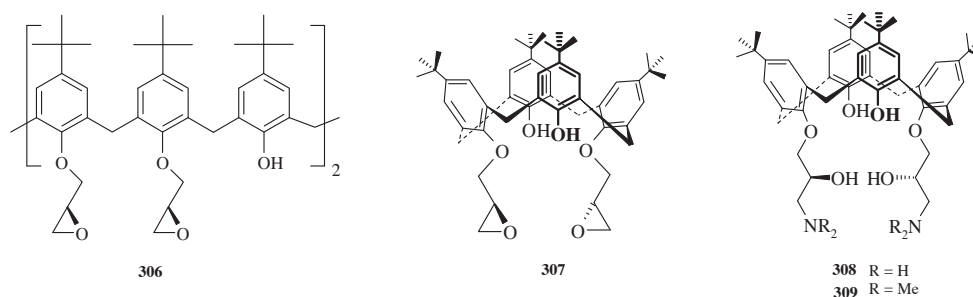
Figure 49. Calixarenes bearing chiral glycidyl groups at the lower rim.
