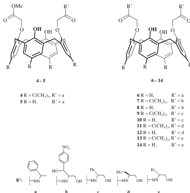
Figure 3. Mono and diamide derivatives of calix[4]arene.
