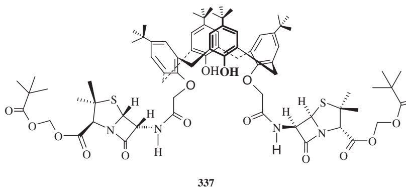
Figure 57. Penicillin grafted p - tert -butylcalix[4]arene.
