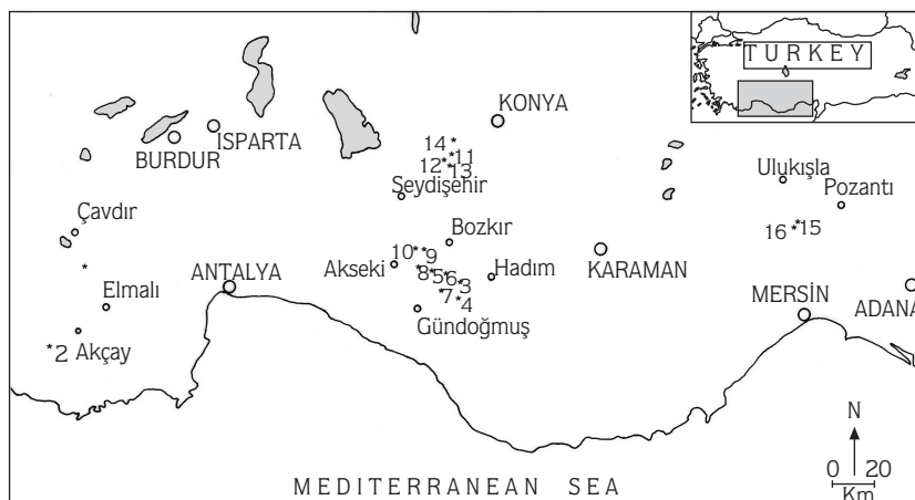
Figure. Geographical situation of the Taurus Mountains and sample stations (from Ustaoglu et al., 2005).
