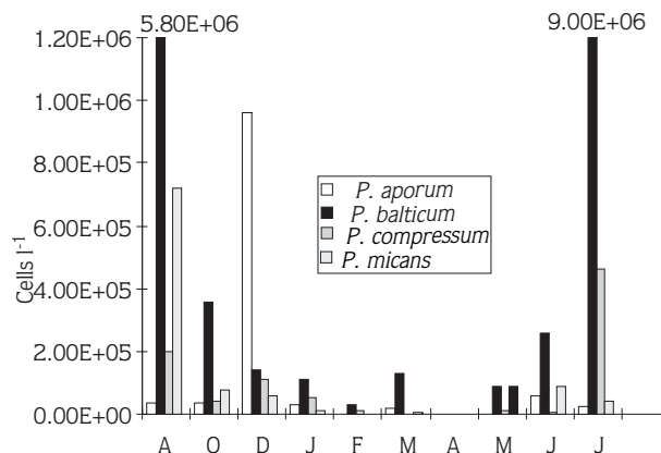
Fig. 11. The annual variations in abundance of Prorocentrum spp. in the southern Black Sea.
