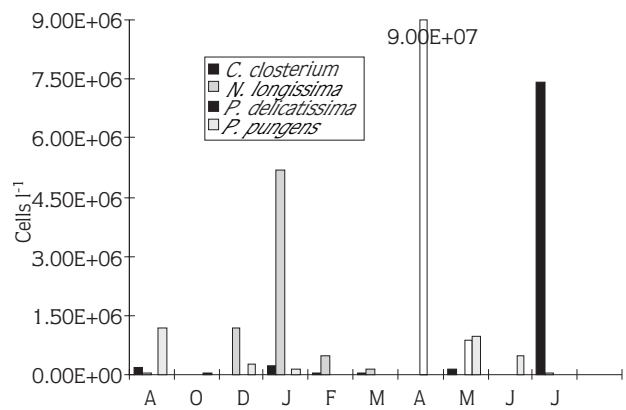
Fig. 9. The annual variations in abundance of some small diatoms in the southern Black Sea.
