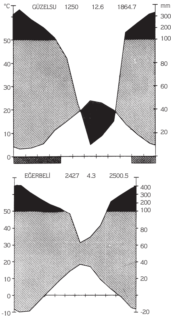
Figure 3. Climate Diagram of Güzelsu and Eğerbeli
