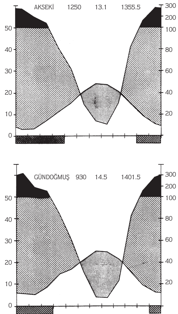
Figure 2. Climate Diagram of Akseki and Gündoğmuş
