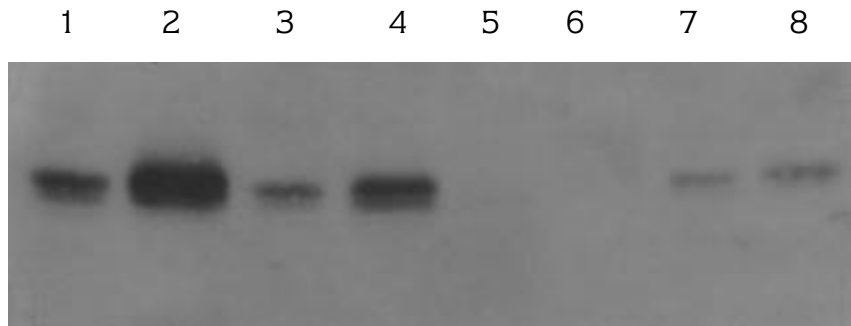
Figure 4. Determination of germin in pellet vs supernatant fractions of homogenates of 3-day-old wheat tissues. Equal quantities of protein from 6-day-old wheat seedlings (1) vascular transition region supernatant, (2) vascular transition region pellet, (3) coleoptile supernatant, (4) coleoptile pellet, (5) leaf supernatant, (6) leaf pellet, (7) root supernatant and (8) pellet were analysed for germin accumulation by electroblotting using antigermine serum.
