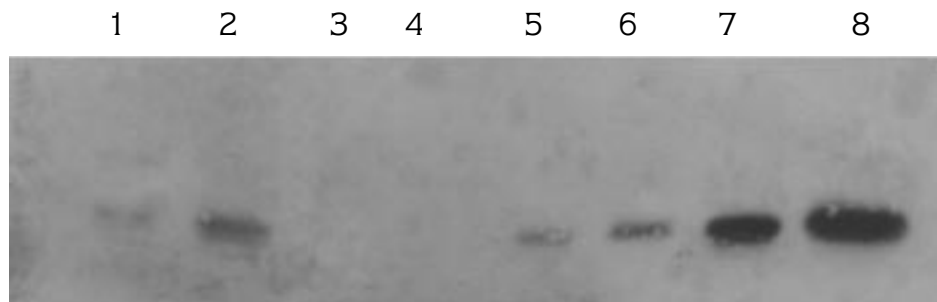
Figure 3. Determination of germin in pellet vs supernatant fractions of homogenates of 3-day-old wheat tissues. Equal quantities of protein from 3-day-old wheat seedlings (1) coleoptile supernatant, (2) coleoptile pellet, (3) leaf supernatant, (4) leaf pellet, (5) root supernatant, (6) root pellet, (7) vascular transition region supernatant and (8) vascular transition region pellet were analysed for germin accumulation by electroblotting using antigemin serum.
