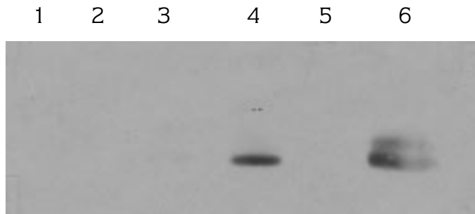
Figure 5. Analysis of germin synthesis in leaves of wheat seedlings grown in darkness and light. Equal quantities of protein from (1) Leaves of 4-day darkness, (2) Leaves of 4-day light, (3) Leaves of 7-day light, (4) Coleoptiles of 7-day light, (5) Leaves of 7-day darkness and (6) Coleoptiles of 7-day darkness were analysed for germin accumulation by electroblotting using antigermine serum.
