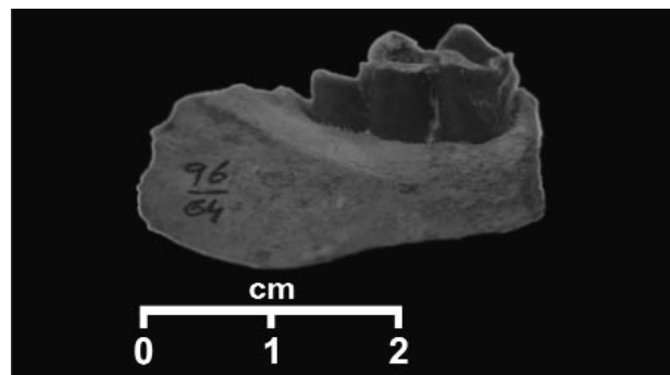
Figure 3. D. majus (PUPC 96/64): Fragment of a right mandibular ramus with M 3 ; buccal view.
