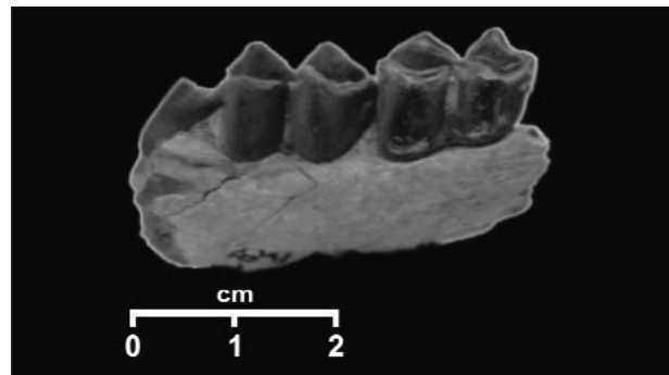
Figure 2. D. majus (PUPC 84/115): A part of a right mandibular ramus with M 2-3 ; buccal view.
