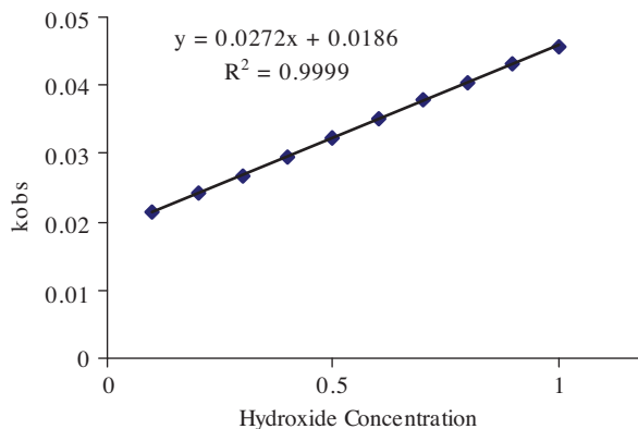
Figure 1. Plot of pseudo-first order rate constant k_{obs} against hydroxide ion concentration.
