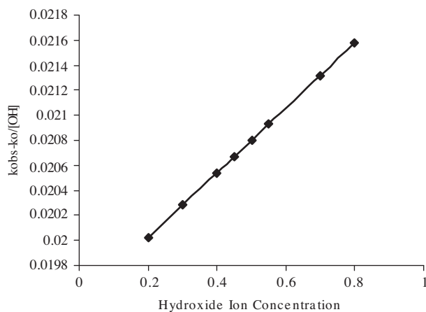
Figure 2. Plot of k_{obs} - k_o/[OH^-] versus [OH^-] for the hydrolysis of 3-(2'-chloro-6'-fluorobenzyl)isocoumarin in the presence of aqueous solution of KOH.
