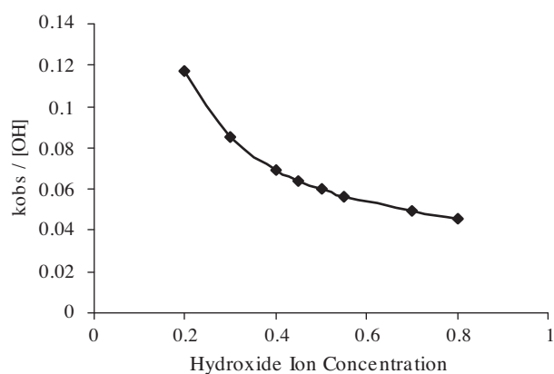
Figure 4. Plot of k_{obs} / [OH^-] vs [OH^-] ignoring k_o for the hydrolysis of 3-(2'-chloro-6'-fluorobenzyl)isocoumarin in the presence of aqueous solution of KOH.
