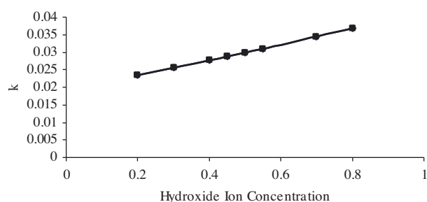
Figure 3. Comparison of the pseudo-first order rate constant k_{obs} with k_{cal} for the hydrolysis of 3-(2'-chloro-6'-fluorobenzyl)isocoumarin in the presence of aqueous solution of KOH.
