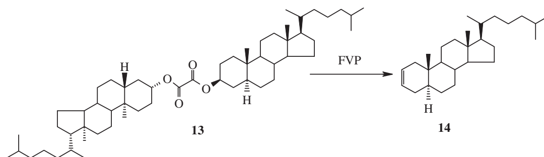
Scheme 7. The FVP of cholestane oxalate dimer (13).
