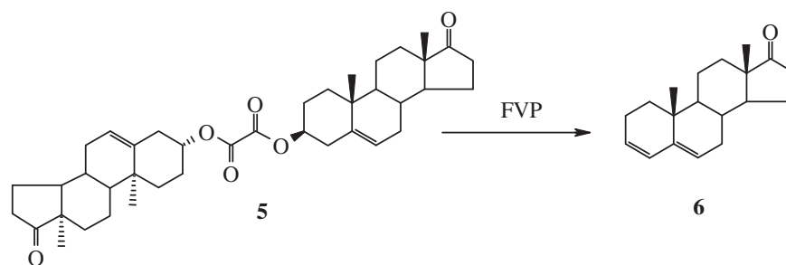
Scheme 3. The FVP of dehydroandrosterone (DHEA) oxalate dimer (5).
