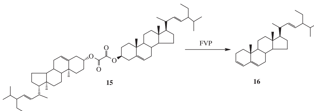
Scheme 8. The FVP of stigmasterol oxalate dimer (15).
