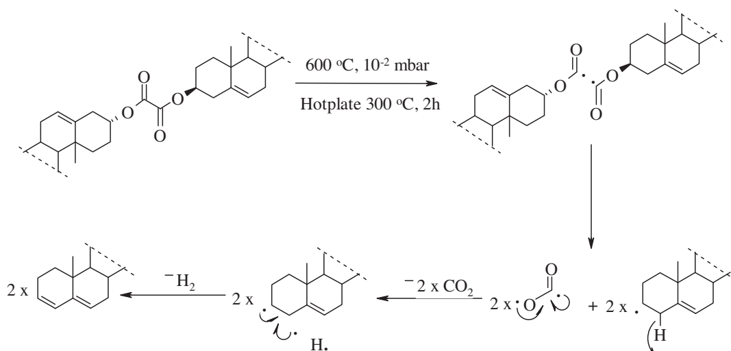
Scheme 9. Possible reaction mechanism for the formation of a double bond via radical.
