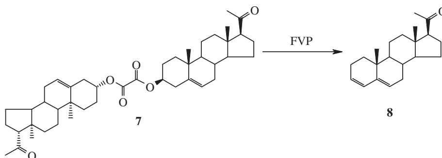
Scheme 4. The FVP of pregnenolone oxalate dimer (7).
