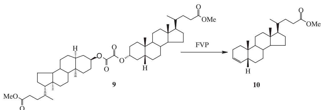
Scheme 5. The FVP of methyl lithocholate oxalate dimer (9).
