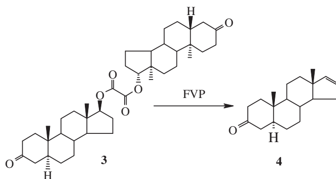
Scheme 2. The FVP of 5 \alpha -testosterone oxalate dimer (3).
