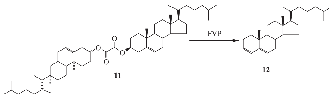
Scheme 6. The FVP of cholesterol oxalate dimer (11).
