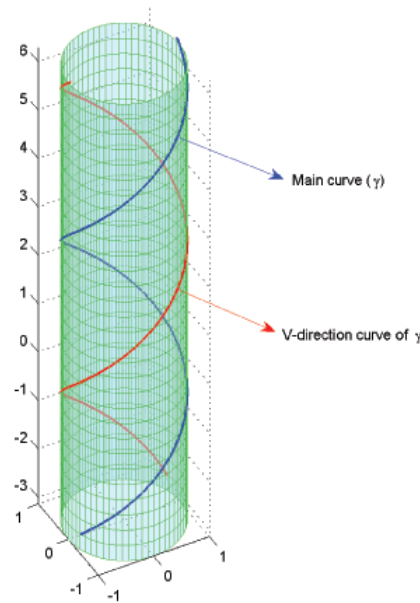
Figure 3. V-direction curve of a cylindrical helix ( c_2 = 0 ).
