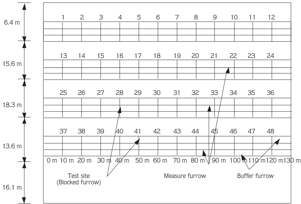
Figure 1. A plan view showing the general layout of the experimental field.
