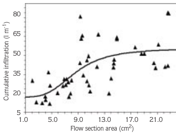
Figure 5. Cumulative infiltration versus flow section area.
