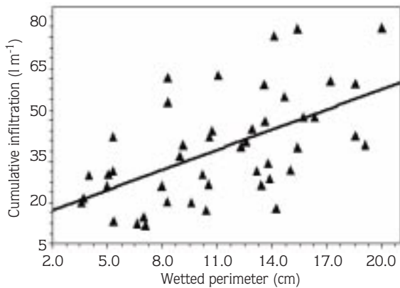
Figure 6. Cumulative infiltration versus wetted perimeter.
