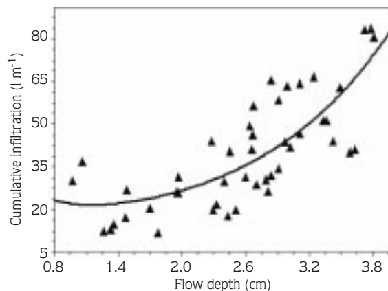
Figure 3. Cumulative infiltration versus flow depth.
