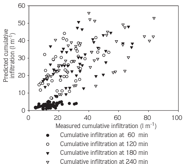
Figure 9. Measured cumulative infiltration versus predicted cumulative infiltration.
