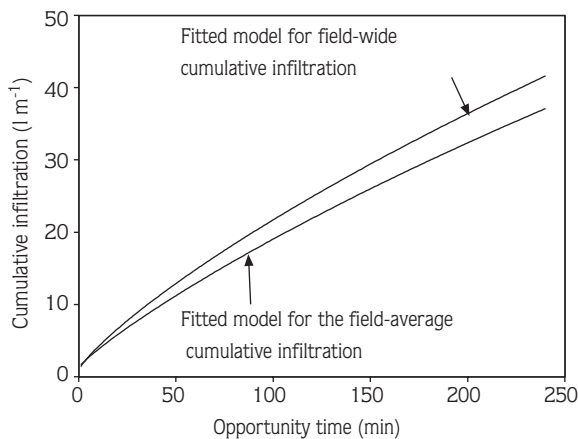
Figure 2. Cumulative infiltration versus opportunity time.
