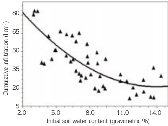
Figure 4. Cumulative infiltration versus initial soil water content.
