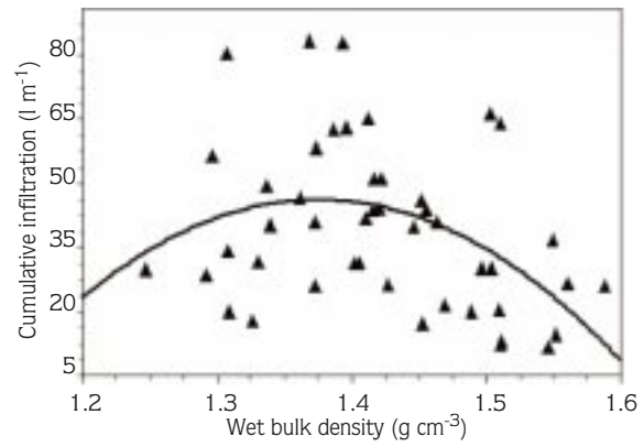
Figure 7. Cumulative infiltration versus wet bulk density.
