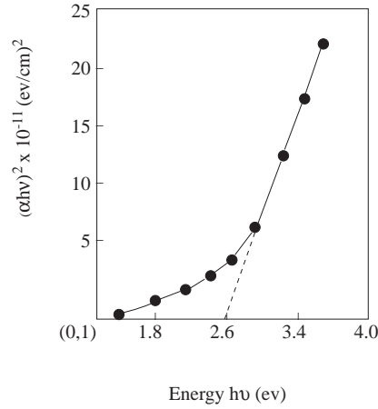
Figure 3. Plot of (\alpha h\nu)^2 versus h\nu for bismuth oxide thin films.
