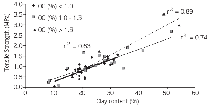
Figure 8. Relationships between aggregate tensile strength and clay contents of soils with different soil organic carbon contents in July, 2003.
