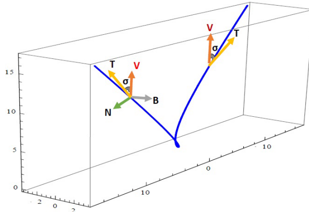
Figure 7. Spacelike B-magnetic curve.
