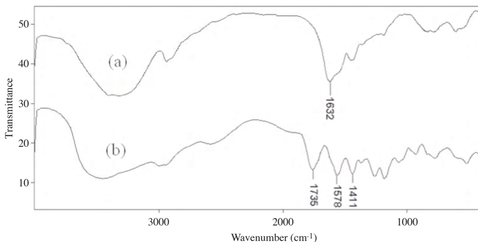
Figure 2. FTIR spectra of starch (a) and starch- g -poly(AA- co -HEMA) hydrogel (b).
