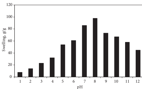
Figure 4. Effect of pH of solution on swelling of starch- g -poly(AA- co -HEMA) hydrogel.
