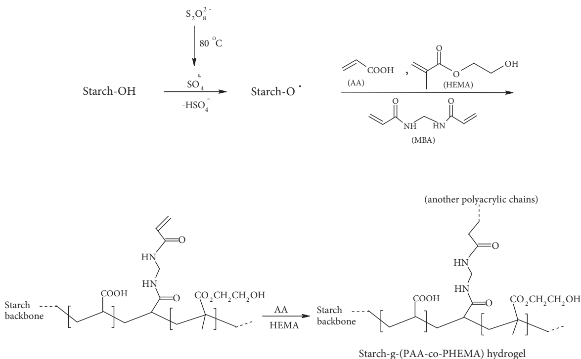
Scheme. Proposed mechanistic pathway for synthesis of the starch-based hydrogels.
