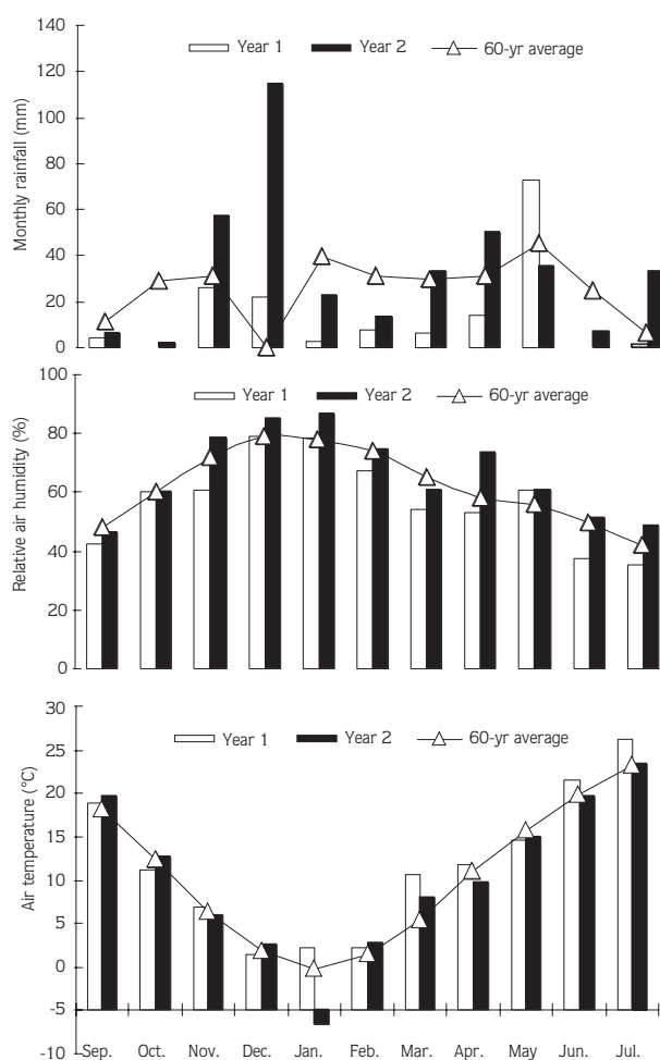
Figure 1. Total monthly rainfall, relative air humidity and mean air temperature during the 2000-2001 and 2001-2002 growing seasons and the 60-year average for the experimental site at Konya, Turkey.
