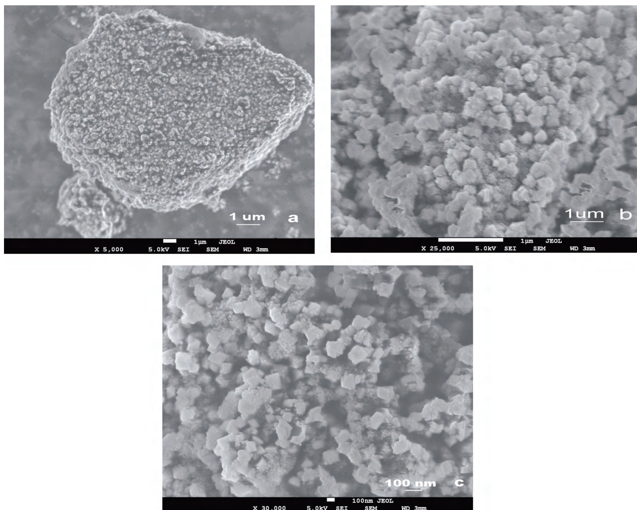
Figure 9. SEM images of cobalt chromite spinel nanocrystals, \text{CoCr}_2\text{O}_4 , obtained at 110\text{ }^\circ\text{C} with different magnifications: a) at \times 5000 , b) at \times 25,000 , and c) at \times 30,000 .
