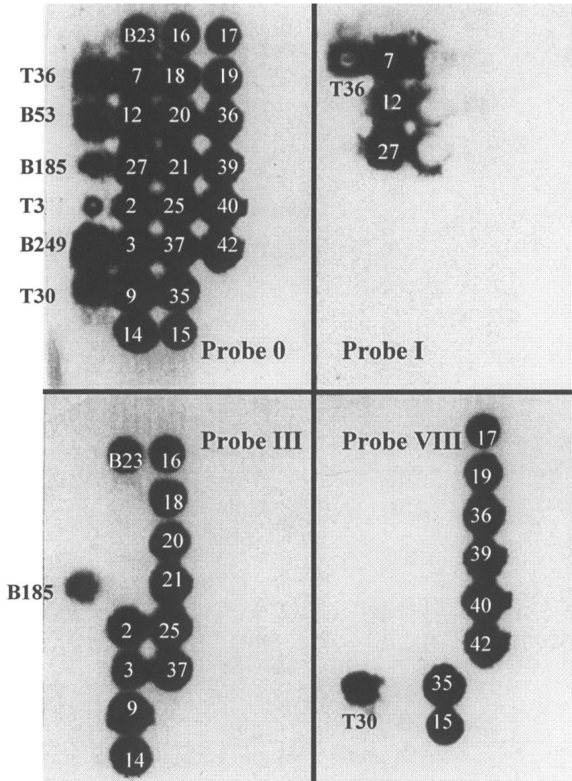
Figure 2. Hybridization of clones obtained from isolate B23. Bold numbers on the left refer to controls and white numbers refer to RT-PCR product of B23 and total 21 clones. Probe 0: RT-PCR product of B23 and the clones reacted with probe 0. Probe I: Clones of 7, 12, and 27, reacted with probe I. Probe III: Clones 2, 3, 9, 14, 16, 18, 20, 21, 25, and 37, reacted with probe III. Probe VIII: Clones 35, 15, 17, 19, 36, 39, 40, and 42, reacted with probe VIII.
