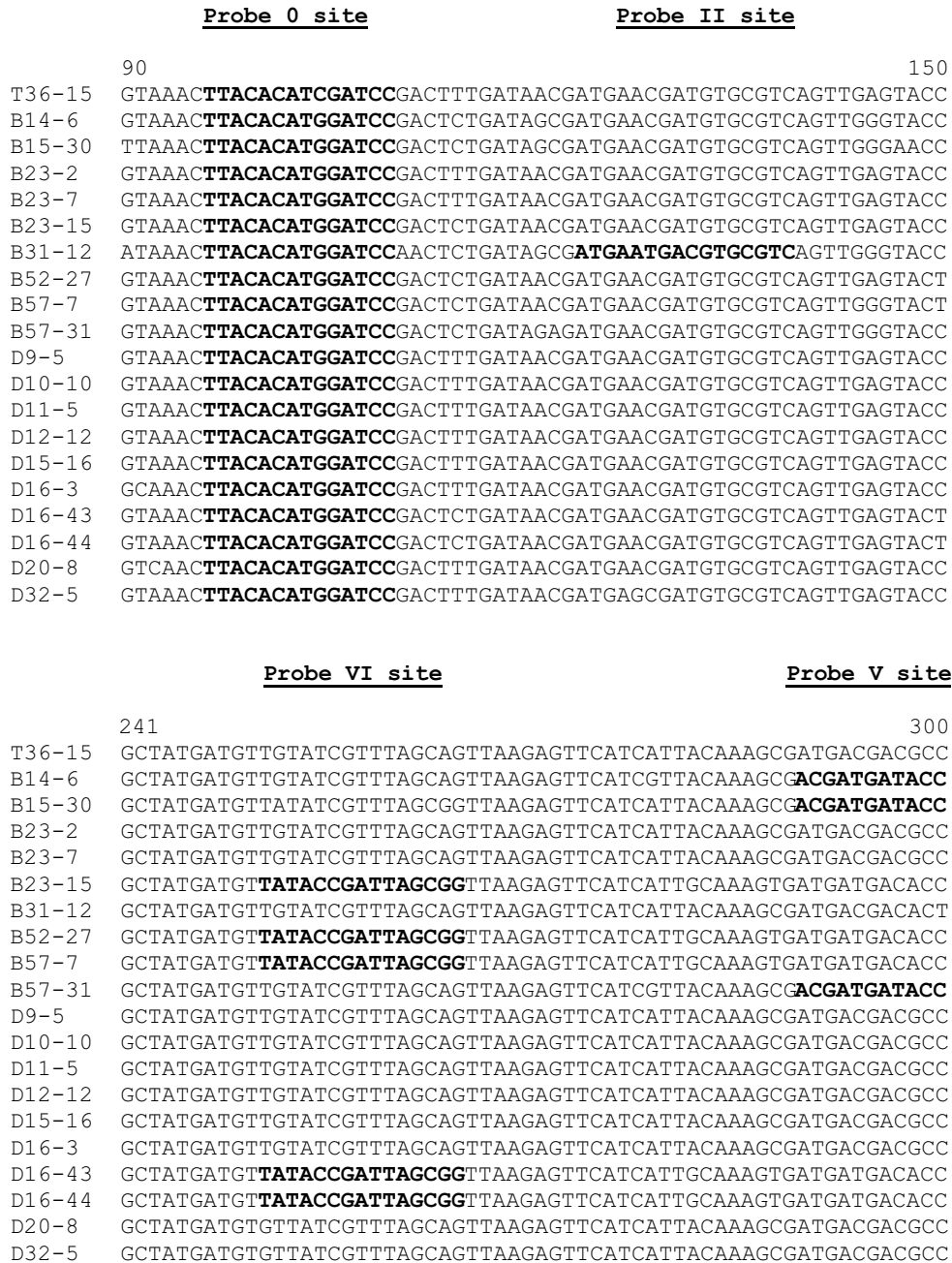
Figure 1. Multiple alignment of the nucleotide sequences of the CPGs of several CTV isolates, showing probe sites. The sequence from reacting with specific probe is highlighted.
