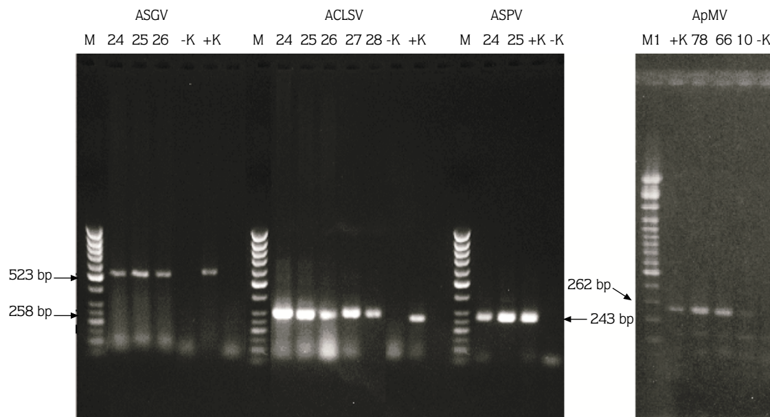
Figure 3. Representative results for the detection of Apple stem grooving virus (ASGV), Apple chlorotic leaf spot virus (ACLSV), Apple stem pitting virus (ASPV) and Apple mosaic virus (ApMV) by RT-PCR. M: 50 bp DNA ladder; M1: 100 bp DNA ladder Plus (Fermentas GmbH Germany); Lanes 24, 25, 26, 27, 28: Apple tree samples from Pozanti-Adana; 78: Granny Smith from Ankara; 10, 66: Golden from İçel; +K: Positive control sample for ASGV, ACLSV, ASPV and ApMV; - K: Water control.
