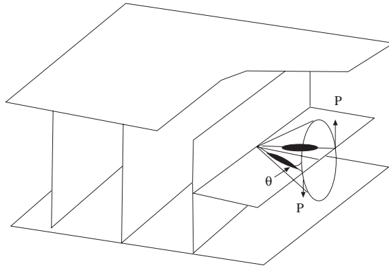
Figure 3. Schematic representation of the FLC cell in the surface stabilized state.
