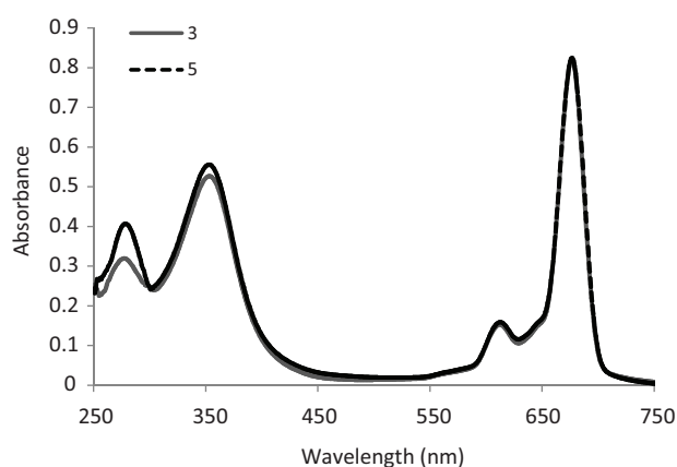
Figure. Absorption spectra of compound 3 and 5 in THF.
