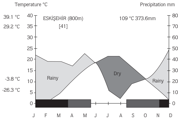
Figure 2. Ombrothermic diagrams of Eskişehir.
