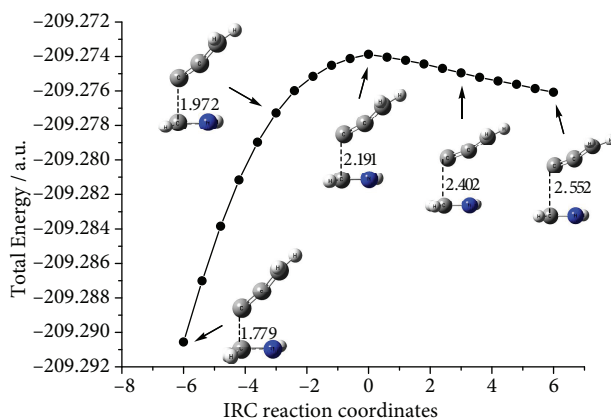
Figure 3. IRC of TS and geometry evolution.
