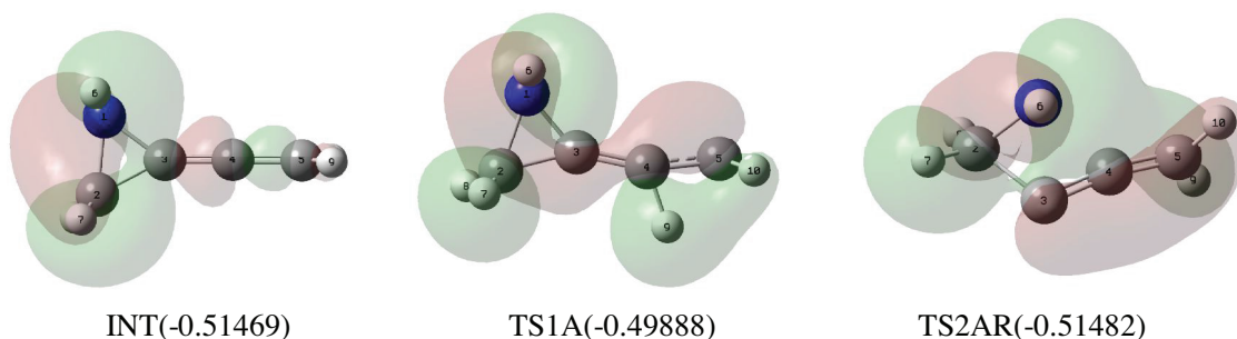
Figure 5. The calculated HOMO - 3 orbitals for INT, TS1A, and TS2AR (from left to right), where the data in parentheses refer to the corresponding orbital energies (in a.u.).
