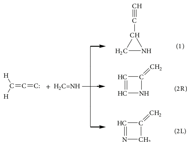
Scheme 1. The 3 isomers of \text{C}_3\text{H}_2 .
