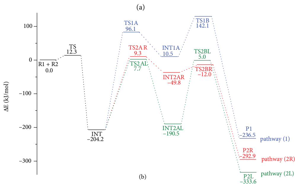
Figure 2. (a): Optimized structures of reactants (propadienyldiene and methyleneimine), transition states, intermediates, and products in the reaction pathway (1) at the MP2 / 6-31 + G* level of theory, where the bond length and bond angle are in angstroms and degrees, respectively. (b): Reaction profile of addition reaction pathways (1), (2R), and (2L) at the CCSD (T) // MP2 / 6-31 + G* level of theory.
