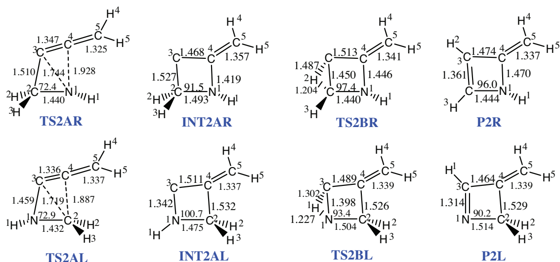
Figure 4. Optimized structures of transition states, intermediate, and products in the reaction pathways (2R) and (2L) at the MP2 / 6 - 31 + G * level of theory, where the bond length and bond angle are in angstroms and degrees, respectively.
