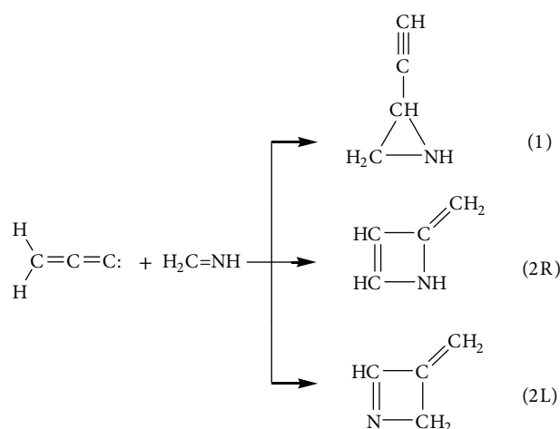
Figure 1. The proposed reaction pathways for the addition reaction between propadienylidene and methyleneimine.
