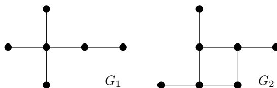
Figure 1. G_1 : 2,2 dimethyl butane and G_2 : 1,2,3 trimethyl cyclobutane.
