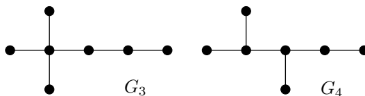
Figure 2. G_3 : 2,2 dimethyl pentane and G_4 : 2,3 dimethyl pentane.
