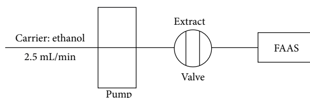
Figure 1. Schematic diagram of the flow injection system coupled to flame atomic absorption spectrometry.
