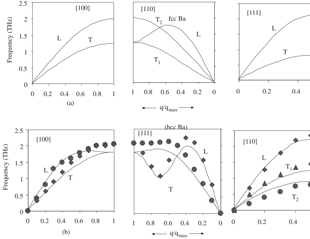
Figure 1. Phonon Dispersion Curves for a) fcc Ba and b) bcc Ba
