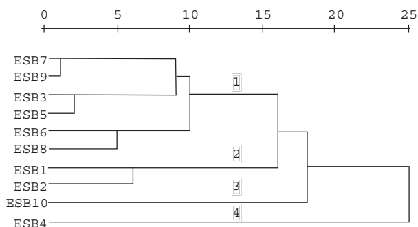
Figure 2. UPGMA dendrogram showing the relationships between H. rhamnoides genotypes.
