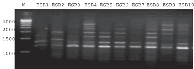
Figure 1. RAPD bands obtained by amplification with primer OPA-1: molecular marker (M).
