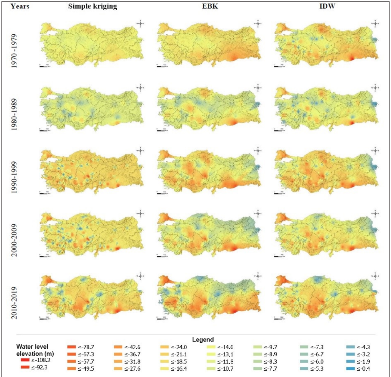
Figure 12. Groundwater level elevation changes between 1970 and 2019.
