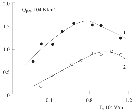
Figure 2. Accumulated charge density in 1- LS and 2- SS samples as a function of polarization intensity.
