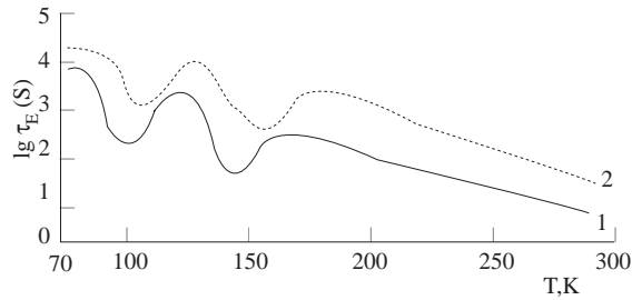
Figure 3. \lg \tau_E PP for various AMS in constant E as a function of temperature. 1. LS.sample, E=0,06 \cdot 10^8 V/m, 2- SS sample, E=0,8 \cdot 10^8 V/m.
