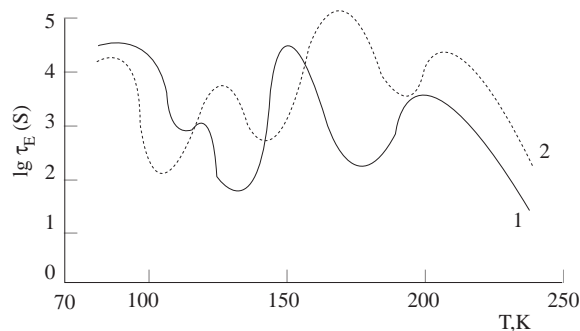
Figure 5. \lg \tau_{\sigma E} PE for various AMS in field E=3 \cdot 10^7 V/m as a function of temperature for samples: 1- LS sample, \sigma=0,050 GPa, 2- SS sample, \sigma=0,070 GPa.
