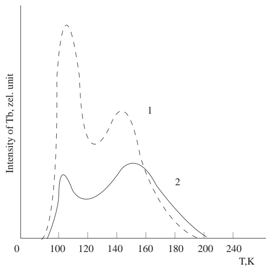
Figure 1. Thermoillustration curves for PP with various AMS,1-LS 2- SS samples.
