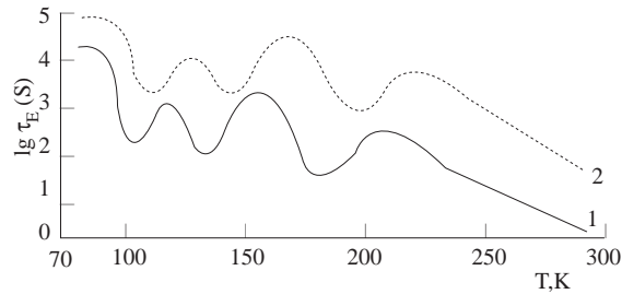
Figure 4. \lg \tau_E PE for various AMS in constant E as a function of temperature. 1- LS sample, E=0,6 \cdot 10^8 V/m, 2- SS sample, E=1,0 \cdot 10^8 V/m.
