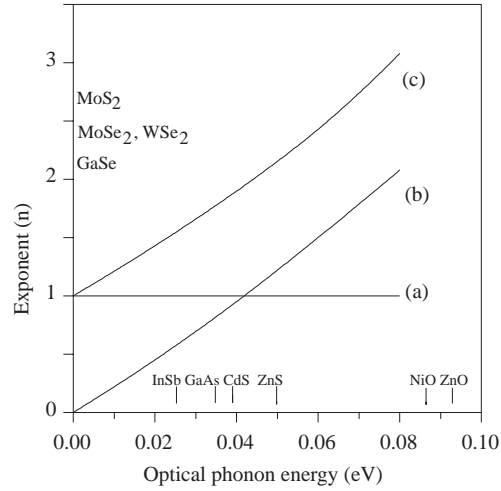
Figure 3. n exponent values as a function of optical phonon energy ( \hbar\omega ) [7].
