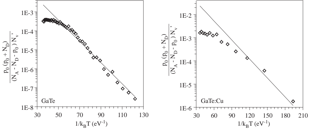
Figure 1. Results of single donor-single acceptor analysis for (a) GaTe and (b) GaTe:Cu samples.
