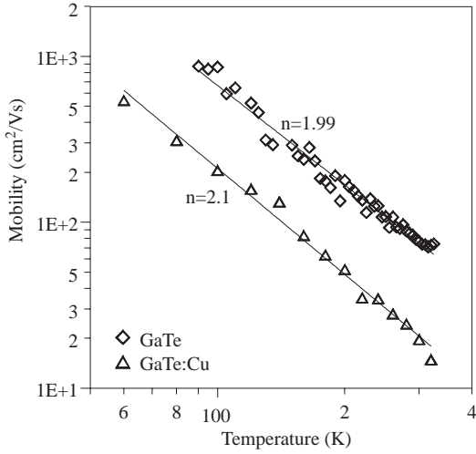
Figure 2. Mobility vs. temperature for GaTe and GaTe:Cu samples.
