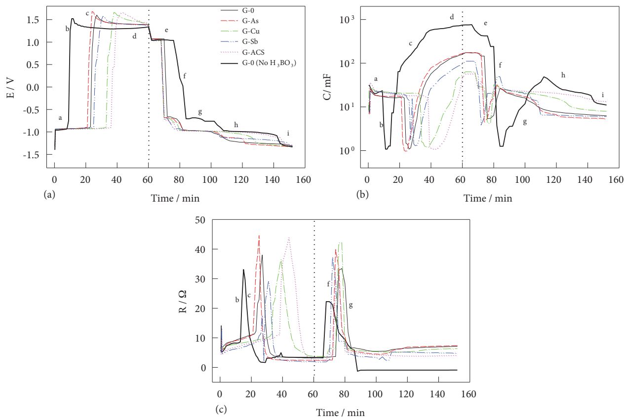
Figure 5. Instantaneous potential, E, capacitance, C, and resistance, R, during the galvanostatic oxidation/reduction of Pb–Ca–Sn alloys at 0.54 mA in 4 M \text{H}_2\text{SO}_4 in the presence of 0.4 M \text{H}_3\text{BO}_3 acid. Bold lines refer to alloy G 0 in the absence of \text{H}_3\text{BO}_3 . The vertical dotted line refers to the start of reduction.
