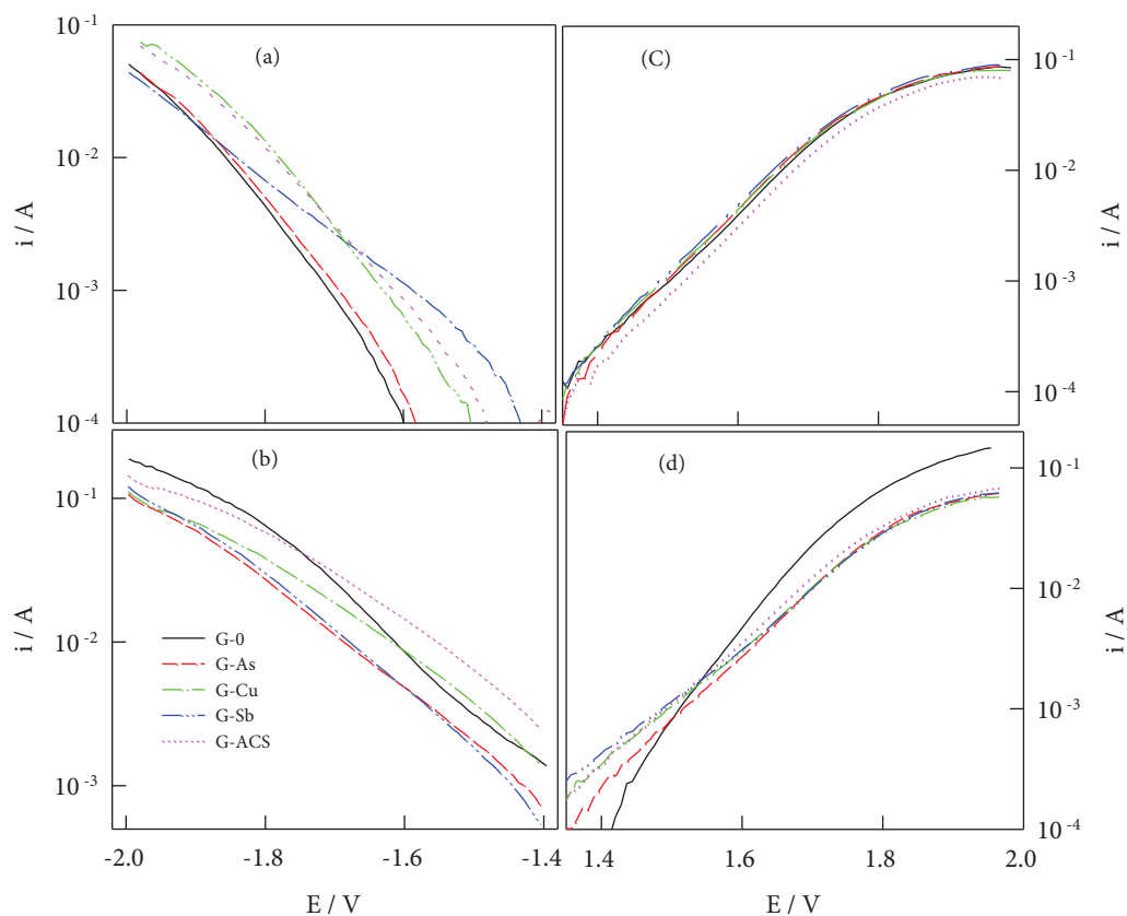
Figure 3. Cathodic polarization curves of hydrogen evolution reaction (a and b) and anodic polarization curves for oxygen evolution (c and d) on Pb–Ca–Sn alloys in 4 M H_2SO_4 in the absence (a and c) and the presence of 0.4 M H_3BO_3 acid (b and d).
