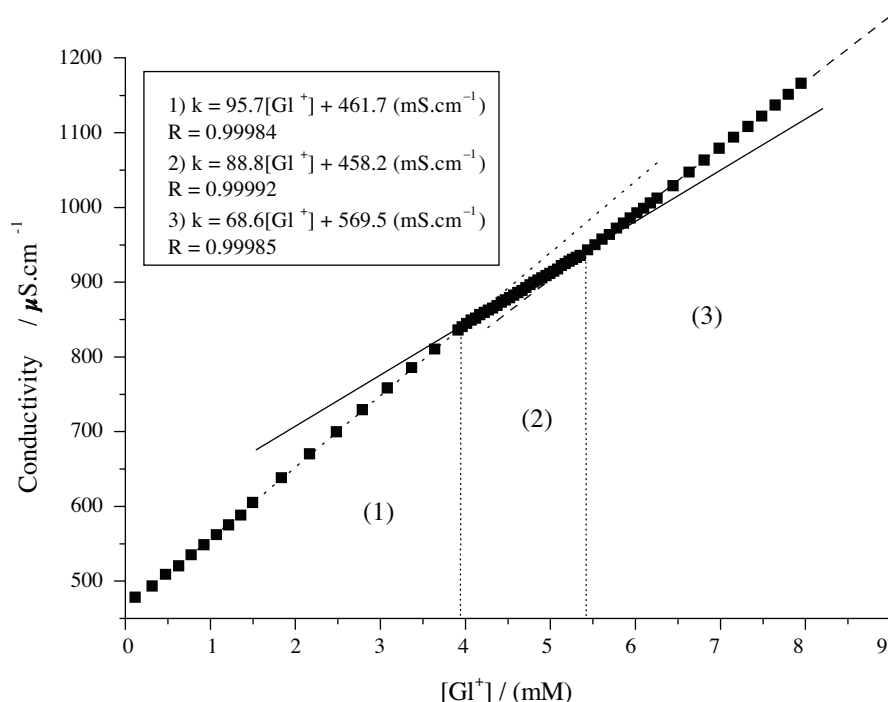
Figure 7. Conductometric titration of \text{G1}^+ 65.0 mM into cell charged with 25.0 mL of SDS 7.7 mM at 298 K.
