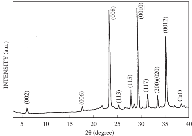
Figure 1. X-ray diffraction pattern of superconducting Bi-Sr-Ca-Cu-O whiskers
