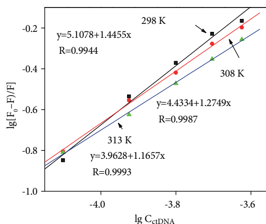
Figure 4. Curves of \lg[(F_0 - F)/F] vs. \lg(C_{ct-DNA}) for MOX-ct-DNA system at different temperatures. C_{MOX} = 0.5 \times 10^{-6} \text{ M} , C_{ct-DNA} = (0.8, 1.2, 1.6, 2.0, 2.4) \times 10^{-4} \text{ M} .
