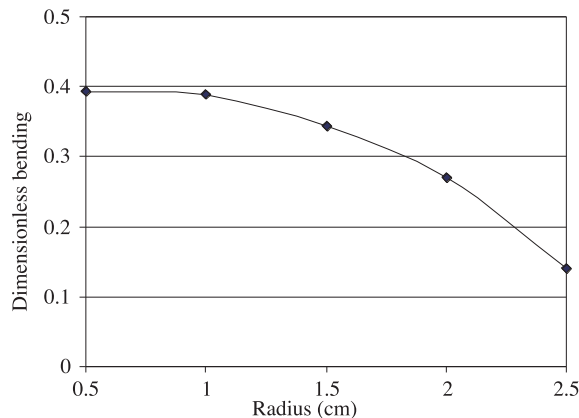
Figure 3. Effect of different crucible radius on the crystallization isotherm for Pe = 1 (absolute values of the dimensionless bending are used).
