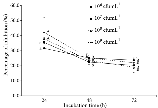
Figure 4B. The percentage of inhibition (%) against E. tarda by various cell densities ( 10^6 , 10^7 , 10^8 , and 10^9 cfu/mL) of L. lactis subsp. lactis CF4MRS at 24, 48, and 72 h. Mean values with same letters within cell densities are not significantly different ( HSD_{0.05} ). Vertical bars indicate standard deviation of means.
