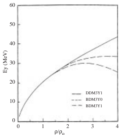
Figure 1. Spin symmetry energy as a function of the relative density \rho/\rho_0 for cold PNM, using different density dependent M3Y interaction.
