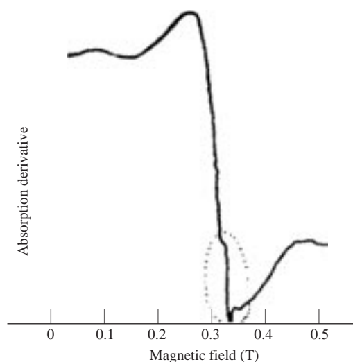
Figure 4. EPR spectrum of \text{Se}_{0.95}\text{As}_{0.05}\text{Cl}_{0.001} , \gamma -irradiated at 77 K ( \text{Co}^{60} , dose 10^7 Rad).
