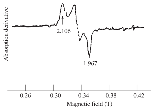
Figure 3. EPR spectrum of Se_{0.95}As_{0.05}Br_{0.1} , \gamma -irradiated at 77 K ( Co^{60} , dose 10^7 Rad).
