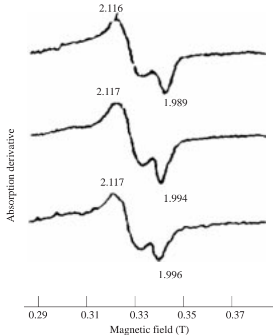
Figure 1. EPR spectra of \text{SeCl}_x , \gamma -irradiated at 77 K ( \text{Co}^{60} , dose 10^7 \text{ Rad} ; 1,2 and 3 at x=0.001 ; 0.01 and 0.1, respectively).
