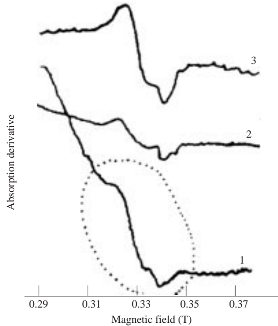
Figure 2. EPR spectra of Se (1), Se_{0.95}As_{0.05}Cl_{0.01} (2) and Se_{0.95}As_{0.05}Cl_{0.1} (3), \gamma -irradiated at 77 K ( Co^{60} , dose 10^7 Rad).
