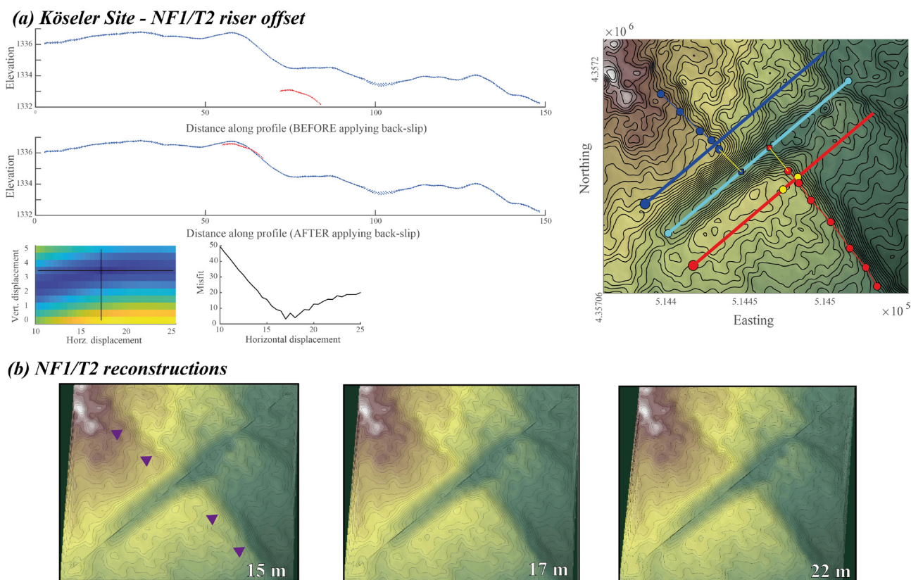
Figure 8. LaDiCaoz analysis of NF1/T2 offset. (a) shows the before/after back-slip of fault-parallel profiles projected on the fault plane, whereas the map on the right presents the location of profiles and orientation of the reference feature, NF1/T2 riser in this case. (b) Incremental offset reconstructions for 15, 17, and 22 m, which all make the min and max boundaries of our boxcar slip model in our calculations.
