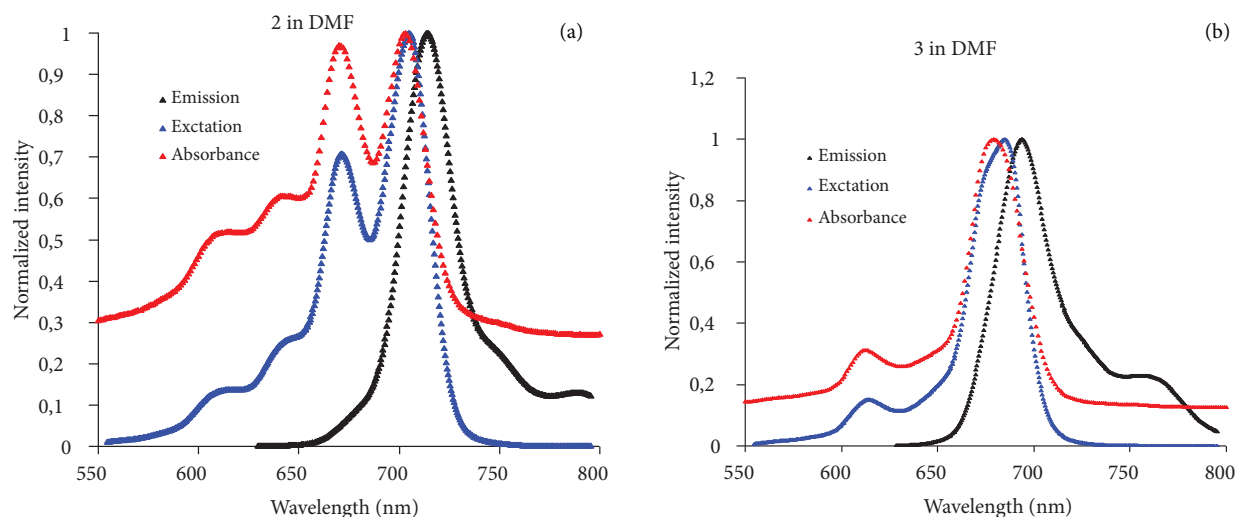
Figure 4. Absorption, excitation, and emission spectra for compounds 2 and 3 . Excitation wavelength = 615 nm in DMF.
