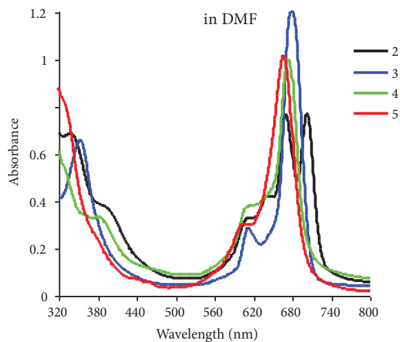
Figure 2. Absorption spectra of 2–5 in DMF at concentrations of \sim 1.2 \times 10^{-5} .
