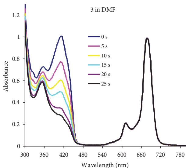
Figure 5. A typical spectrum for the determination of singlet oxygen quantum yield. This determination was for compound 3 in DMF at a concentration of 1 \times 10^{-5} mol \text{dm}^{-3} .
