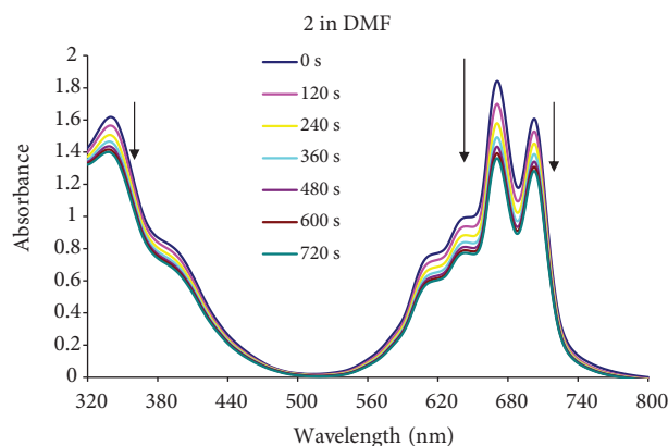
Figure 6. The photodegradation of compound 2 in DMF showing the disappearance of the Q band at 2-min intervals.
