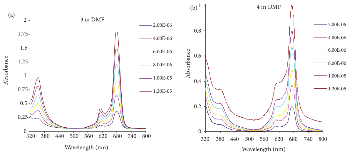
Figure 3. Absorption spectral changes of 3 (a) and 4 (b) in DMF at different concentrations: 2 \times 10^{-6} (A), 4 \times 10^{-6} (B), 6 \times 10^{-6} (C), 8 \times 10^{-6} (D), 10 \times 10^{-6} (E), 12 \times 10^{-6} mol dm ^{-3} .
