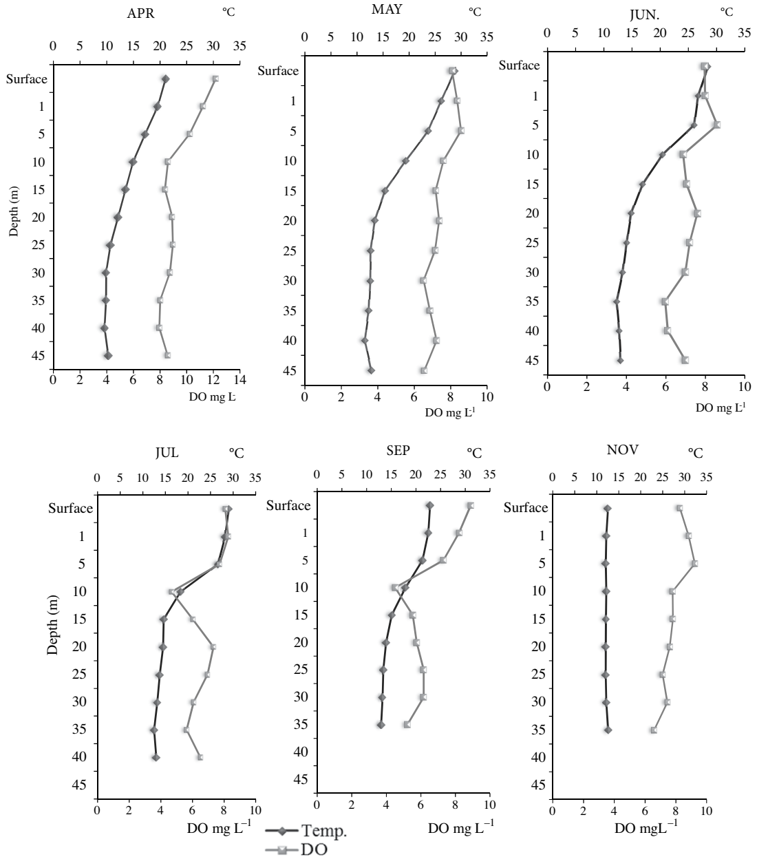
Figure 2. Vertical profiles (every 5 m of depth) of temperature ( ^{\circ}\text{C} ) and dissolved oxygen ( \text{mg L}^{-1} ) in the study area. Illustrations were formed for the vertical zooplankton sampling period.
