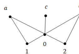
\Gamma_I(X)
