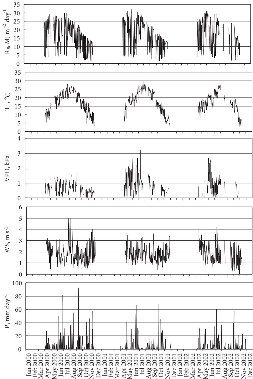
Figure 3. Climate data for the red pine forest in the measured years. From the top, the daily total solar radiation ( R_s ), the daily mean air temperature ( T_a ), the daily mean vapor pressure deficit (VPD), the daily mean wind speed (WS), and the daily rainfall (P).
