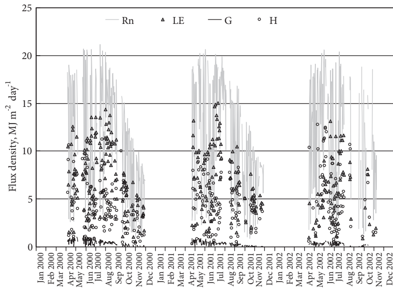
Figure 5. Energy fluxes for the growing seasons of the measured years, calculated using the Bowen ratio-energy balance (BREB) approach. The net radiation ( R_n ) can be seen together with its division into the sensible heat flux (H), the latent heat flux (LE), and the ground heat flux (G). All fluxes may be read on the y-axis.
