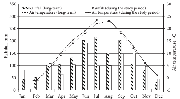
Figure 2. Monthly rainfall (mm) and average air temperature (°C) during the study period (2000-2002). The hashed bars and dashed line indicate the long-term (1985-2008) monthly averages.
