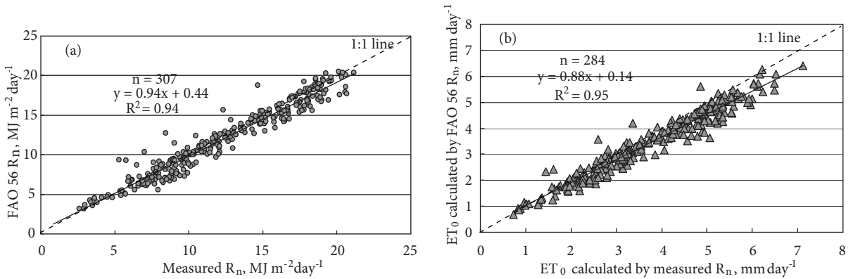
Figure 4. a) Net radiation ( R_n ) estimated from FAO-56 daily time step equations against the measured R_n at the study site and b) correlation between the reference evapotranspiration ( ET_0 ) by the measured R_n and by that of the estimated R_n through FAO-56; n = number of measured days.
