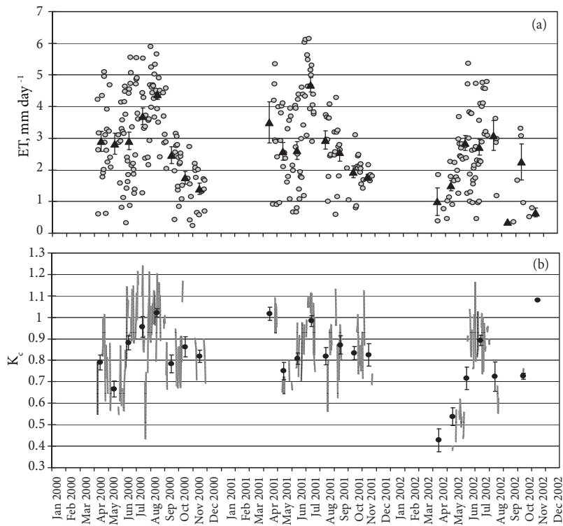
Figure 6. a) Changes in the daily average estimates of evapotranspiration (ET) from the red pine forest using the Bowen ratio-energy balance (BREB) approach and b) daily crop coefficients ( K_c ), i.e. the ET:ET_0 values. Bars are standard errors of the mean monthly ET and K_c values.
